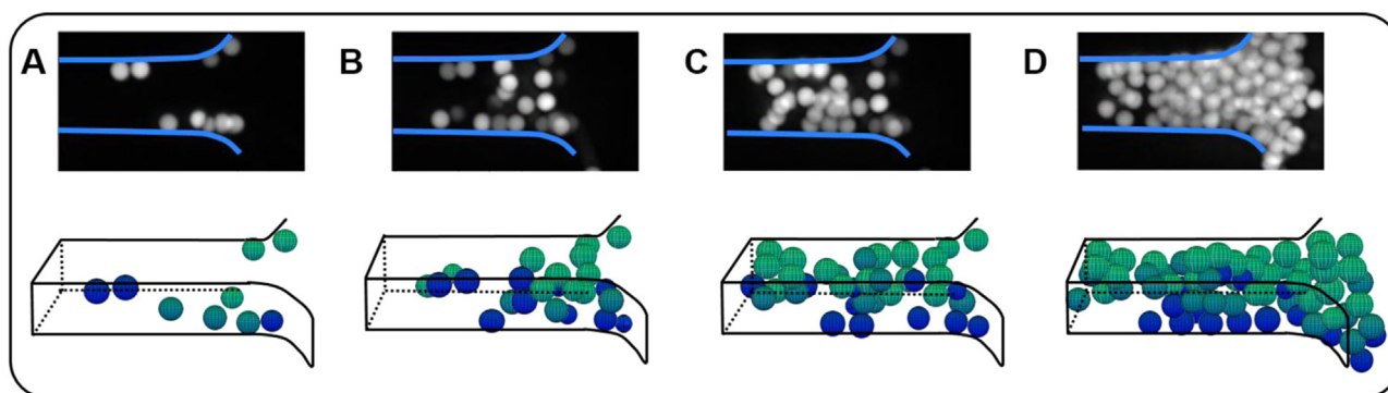
Fig. 4. A–D Confocal image of a pore progressively fouled by the deposition of colloidal particles. (top) Z-Projection (projection on one plan) of all the images taken during a z-stack of a pore. (Bottom) Corresponding reconstruction, after image analysis, of the deposit. Particles are depicted according to a blue-green color gradient representative of their vertical position (dark blue: particle on the floor; green: particle on the roof). The flow goes towards the left (For interpretation of the references to color in this figure legend, the reader is referred to the web version of this article).
