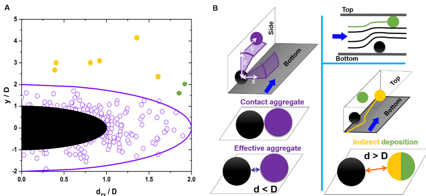
Fig. 11. A-Distance of deposition downstream from the static particle in the flow direction ( y ) vs. the distance in zx plane, perpendicular to the flow. The black area is the location of the particle already attached on the pore walls. The area delimited by the purple circle corresponds to the aggregation zone where final distances d between the two particles, in both planes ( zx and zy ), are smaller than D . Some particles will deposit further away from the static particle (yellow and green points). B-Characteristics of the deposition of a newly captured particle (purple, yellow or green particles) on to the pore walls after its interaction with the closest particle already deposited on the pore surface (the black particle). Purple particles are captured at a distance smaller than D , forming either a true (contact) or an effective aggregate. Some particles will deposit further away from the static particle (yellow and green). Yellow ones correspond to particles being deposited after crossing an immobile particle but at a distance greater than D (middle scheme on the right). Green particles get attached on the same lateral side and the opposite corner (top right corner scheme). Such particles experience a local constriction along the channel height due to the immobile particle in the opposite corner (For interpretation of the references to color in this figure legend, the reader is referred to the web version of this article.).
