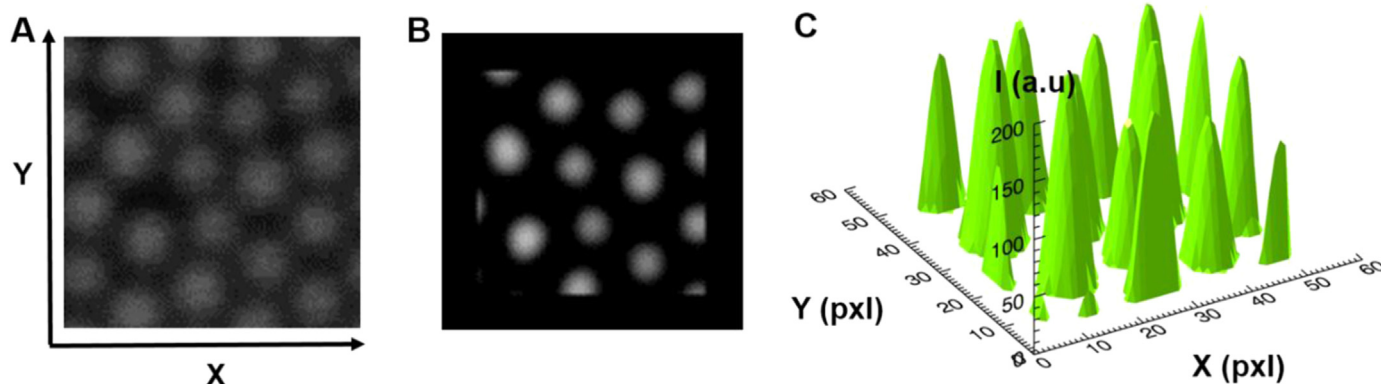
Fig. 2. A-Raw confocal image of spherical colloids. B-The image in A after a spatial band pass filtration. C-Intensity surface plot of the image B.
