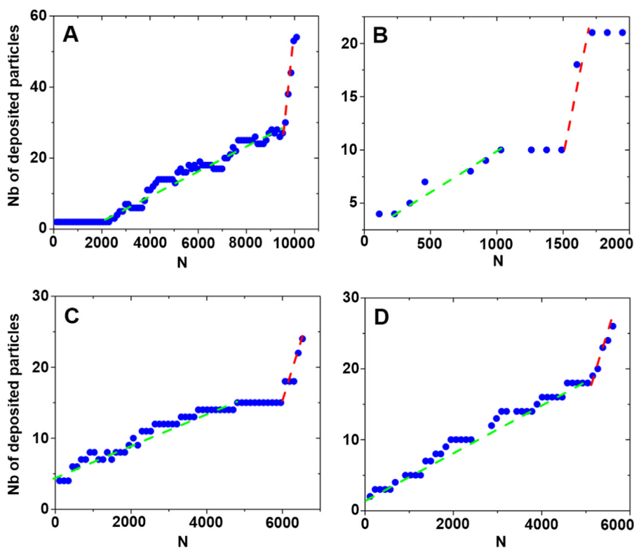
Fig. 8. (Top) Dynamics of particle capture for four different pores. Experiments were performed within a W = 16 \mu\text{m} and H = 12 \mu\text{m} channel with 4 \mu\text{m} particles at a volume fraction equal to 5 \cdot 10^{-5} and \Delta P = 30\text{mbar} . The green and red dashed lines correspond to linear fits of the data in the first and the second step, respectively. Different views of the clog structure at the end of each of these experiments are provided in Fig. 7 (bottom part). In the two Figs. 7 and 8 the same label corresponds to the same experiment (For interpretation of the references to color in this figure legend, the reader is referred to the web version of this article.). (For interpretation of the references to color in this figure legend, the reader is referred to the web version of this article.).
