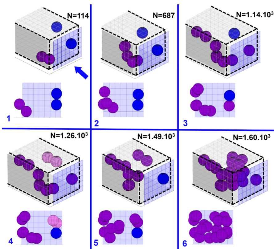
Fig. 14. 3D images of the clog buildup corresponding to the deposition curve in Fig. 8B. In each image, blue particles are isolated, while pink and purple ones belong to two different aggregates. The arrow indicates the flow direction (For interpretation of the references to color in this figure legend, the reader is referred to the web version of this article.).
