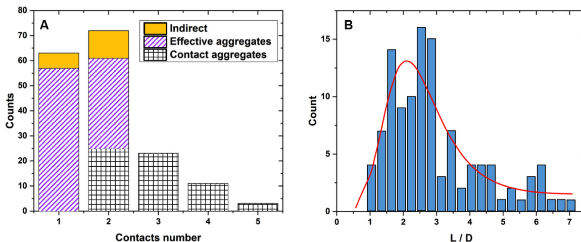
Fig. 12. A-Distribution of the number of contacts for the particles belonging to the first layer in all the considered pores. The definition of each category is in Fig. 11B. These numbers do not include the contact with the pore surface. B-Distribution of the deposition lengths from the pore entrance for particles having interacted with a deposited particle or an aggregate. The (red) line is a log-normal fit of the data peaked around 2.1 L/D (For interpretation of the references to color in this figure legend, the reader is referred to the web version of this article.).
