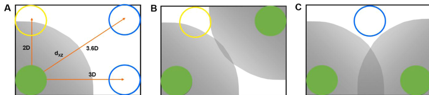
Fig. 10. A-Cross section of a pore when a particle is captured in one corner (green). The grey quarter of circle, with a radius equal to 2.5D , corresponds to the range of hydrodynamic interaction (HI) created by the captured particle. Top and bottom right corners are the only eligible corners for direct capture positions (blue circles). A particle in the top left corner (yellow circle) would experience HI from the captured one, as would all incident particles within the grey zone, and would have their trajectory modified. B and C-Hydrodynamic influence of two particles captured on corners on opposite sides of the pore. We clearly see that it is only when both captured particles are on the same horizontal wall that incident particles can flow through the pore without experiencing HI from the already captured particles (For interpretation of the references to color in this figure legend, the reader is referred to the web version of this article.).
