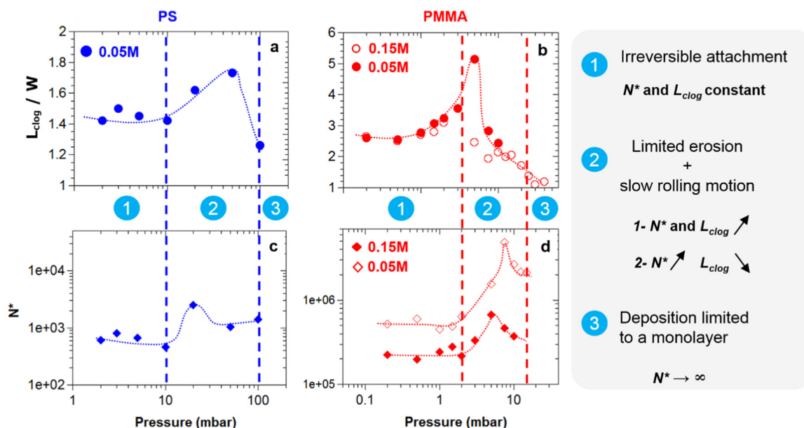
Fig. 5. Evolution of N^* and L_{clog} with the applied pressure difference, for 2 \mu\text{m} PS and 4 \mu\text{m} PMMA particles inside a pore with a width equals to 8 and 18 \mu\text{m} respectively. The dashed lines correspond to the transition between the three clogging regimes. The main features of each regime are summarized on the right panel.
