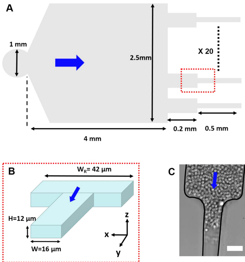
Fig. 1. A-Geometry of the microfluidic model filter. B-Close-up view of the reservoir and the pore entrance zones. C-Top view image of a clogged pore. The black lines correspond to the outlines of the pore. The blue arrows point to the flow direction. The scale bar corresponds to 16 \mu\text{m} (For interpretation of the references to color in this figure legend, the reader is referred to the web version of this article.).
