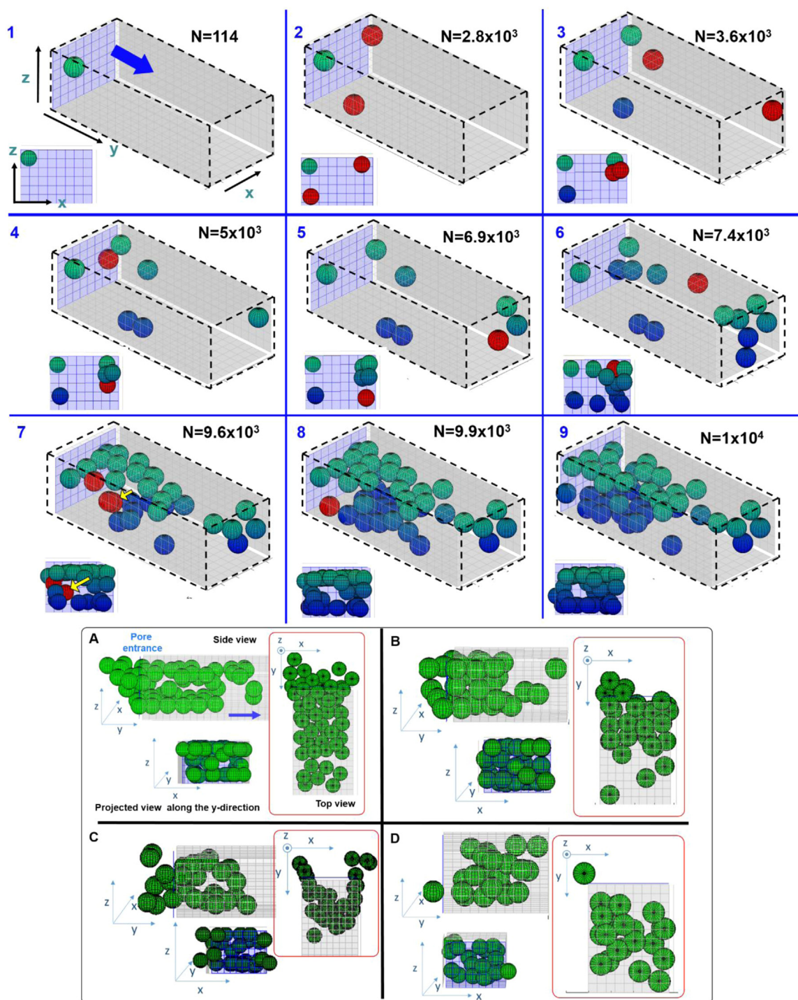
Fig. 7. (Top) 3d images depicting the building-up of the clog. The blue plane represents the cross section at the entrance, and the grey ones the four pore walls. The blue arrow points to the flow direction. The red particles are the freshly captured ones. Particles are depicted according to a blue-green color gradient representative of their vertical position (dark blue: particle on the floor; green: particle on the roof). The projected view, perpendicular to the flow directions helps visualizing the progressive inward fouling. In image 7 the yellow arrow points towards the first particle that gets captured in bulk by immobile particles and not by the surface of the pore. (Bottom) Various 3D views of the clogs obtained at the end of the fouling process for the four trials. The views in top left corner corresponds to the final structure of the clog formation shown in the top part (For interpretation of the references to color in this figure legend, the reader is referred to the web version of this article.).
