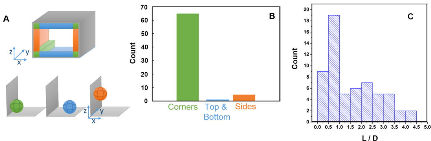
Fig. 9. A-Scheme of the three different zones of particle direct deposition onto the walls of the pore. Particles can deposit on corners (green area), horizontal plates (blue areas) or on side walls. (orange area). B-Proportion of the captured particles in each of these zones. C-Distribution of the positions of the particles captured directly by the pore walls from the pore entrance L , scaled by the particle diameter D (For interpretation of the references to color in this figure legend, the reader is referred to the web version of this article.).
