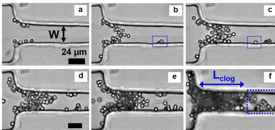
Fig. 6. Images of the clog building-up by 4 \mu\text{m} PMMA particles inside a pore of width W and height H both equal to 24 \mu\text{m} . At the end of the clogging (image f), the isolated aggregate (highlighted by the dotted rectangle) does not partake to the growth of the main clog. L_{clog} is equals to 2.8 W .
