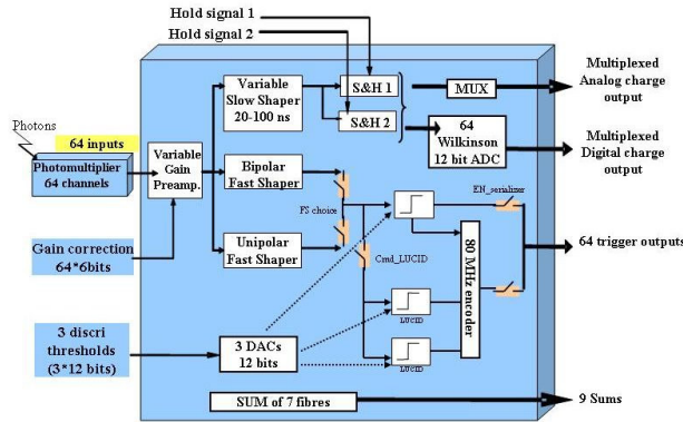
Figure 3: Block diagram of MAROC second version.
