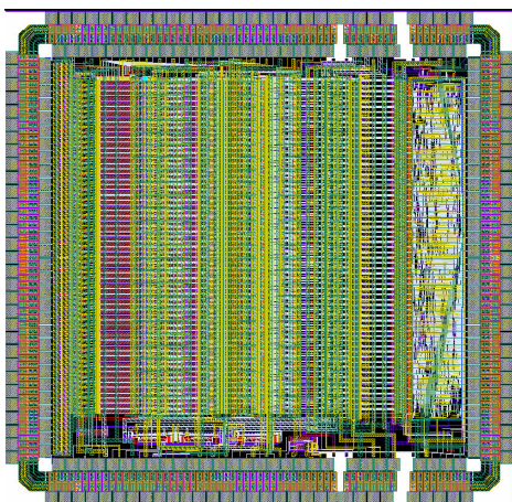
Figure 1: MAROC second version layout.
