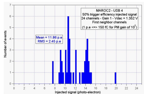
Figure 14: Injected signal for which cross-talk appears.
