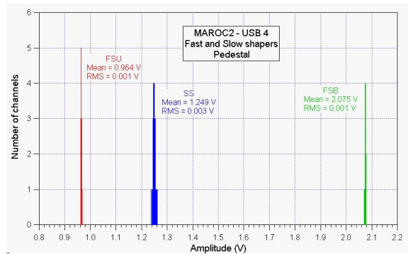
Figure 5: Distributions of fast and slow shapers pedestals (FSU: fast shaper unipolar, FSB: fast shaper bipolar, SS: slow shaper).
