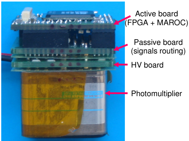
Figure 16: First version of the PMF.
