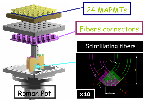
Figure 2: Schematic of a Roman Pot of the ATLAS luminometer.
