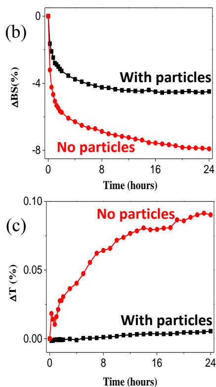
Fig. 2 (a) The bulk phase behavior of the Janus emulsions created by mixing water, silicone oil and sunflower oil. In each panel, the left sample contains \sim 12 mg of silica particles; there are no particles in the right sample. Oil globule aggregation process starts at the top of the right sample (marked black). (b) Time evolution of the backscattering intensity with time ( \Delta BS ) at the lower part (1/3) of the samples in (a). (c) Time evolution of the transmission intensity ( \Delta T ) at the upper part (1/3) of the samples in (a).
