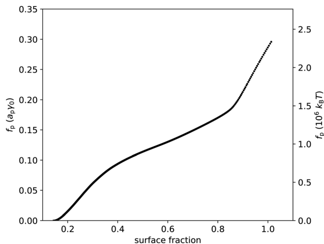
Fig. 3 Free energy per particle \bar{f}_p , in units of a_p \gamma_0 and in units of 10^6 k_B T , vs. surface fraction \phi . This graph was extracted from the data presented in Fig. 2 using eqn (23).
