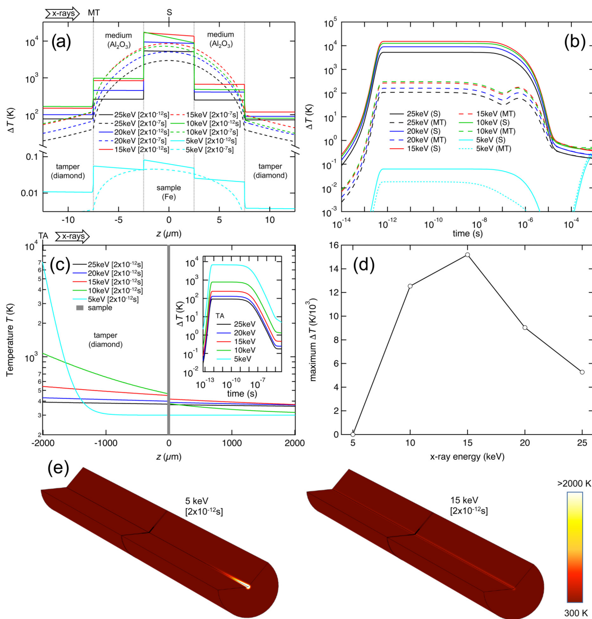
FIG. 5. Variance of the thermal response with x-ray photon energy. (a) Temperature change vs position along the beam path center ( r = 0 ) in the sample region. (b) Temperature change vs time at sample center (S) and leading medium-tamper interface (MT). (c) Absolute temperature vs position along the beam path center ( r = 0 ) across the whole target with inset showing temperature change vs time at the leading tamper free surface (TA). (d) Maximum temperature increase at sample center (S) as a function of photon energy. (e) Cylindrical simulation region temperature immediately after heating for 5 keV (left) and 15 keV (right). The black lines in (a)–(c) correspond to the standard 25 keV simulation results. Times are given in square brackets in seconds.
