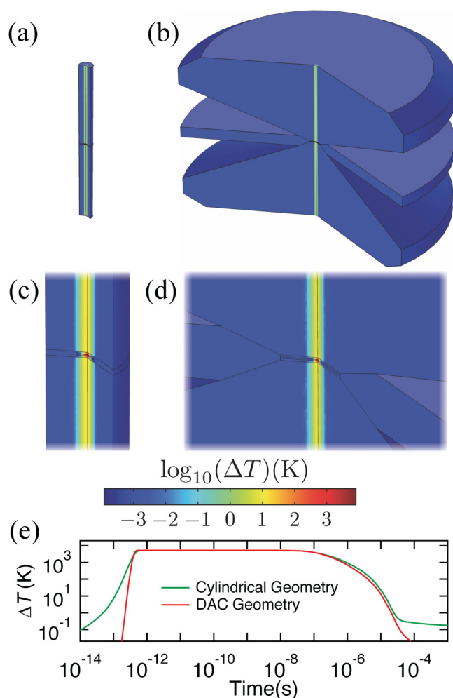
FIG. 15. Comparison between temperature distributions for the main simulation geometry with the standard materials (a) and a comparable simulation for a diamond anvil cell (b). The time of the simulation snapshots in (a)–(d) is 1 \times 10^{-7} s. Close-ups of sample regions (c) and (d) show nearly identical temperature behavior at these early times. A comparison of the temperature history at the sample center shows notable differences in simulated temperature only during heating (a shorter pulse was assumed for the DAC simulation) and very late in the cooling phase. The latter difference is due to the larger heat sink provided by the full-size target assembly, resulting in lower limiting temperature.
