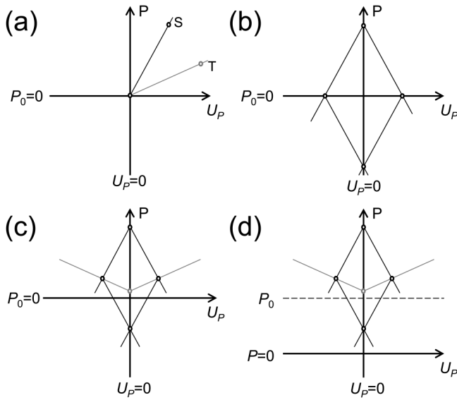
FIG. 11. Impedance match construction for the mechanical evolution of the x-ray heated sample (pressure P vs mass velocity U_p ). Material responses are lines, whereas dots are specific states achieved; S represents the sample and T a surrounding (i.e., tamper) material, presumed to be more weakly heated. Shocks and releases are approximated as linear elastic (i.e., \Delta P \approx \rho c_s \Delta U_p , where \rho is the density and c_s is a wave velocity). Uniform heating in each layer is assumed. (a) Compression and release response of the high-Z sample (S) and a low-Z tamper (T), where the tamper is assumed to also have lower impedance. Lines indicate achievable states on compression from initial state P_0 = 0, U_p = 0 ; the dots represent particular compressed states. (b) Case of a freestanding sample layer in vacuum under x-ray heating. The sample foil is immediately driven to a high thermal pressure at zero velocity, and releases from both sides (Fig. 10), driving each side of the target to plus or minus a particle speed and zero pressure. These release waves converge at target center, causing a further stress reduction equivalent to the initial thermal pressure; i.e., the interacting release waves produce tension, and, if it exceeds the tensile strength of the material, spall. (c) Case of a tamped sample, with only a partial reduction in pressure on initial release due to confinement by surrounding material (Fig. 10), and a reduced but not eliminated tension state (tension is prevented if sample and tamper have closer impedances). (d) While the preceding scenarios (a)–(c) apply for a typical laboratory condition with an initial pressure P_0 much less than the dynamic pressure (i.e., vacuum or ambient initial conditions), this scenario begins at a high initial hydrostatic pressure ( P_0 > 0 ) comparable in magnitude to the dynamic pressure, as is made possible by pre-compression with a strong tamper. 32,48 Achieved pressures are larger, while tension is suppressed.
