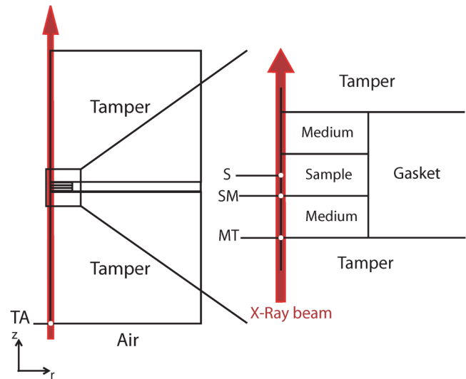
FIG. 1. Schematic illustration of the general model geometry, depicting the axis-symmetric slice from the axis to the edge of the cylinder. For finite element models, a 2D cylindrical geometry 160\ \mu\text{m} in radius and 4005\text{--}4025\ \mu\text{m} in length is employed. For hydrodynamic models, a simple 1D representation of the boxed region is used. X rays are incident from below. Standard dimensions are specified in Table II. Measurements are taken at S (sample center), SM (sample-medium interface), MT (medium-tamper interface), and TA (tamper-air interface) with interfaces referring to the leading (upstream) interface unless otherwise indicated.
