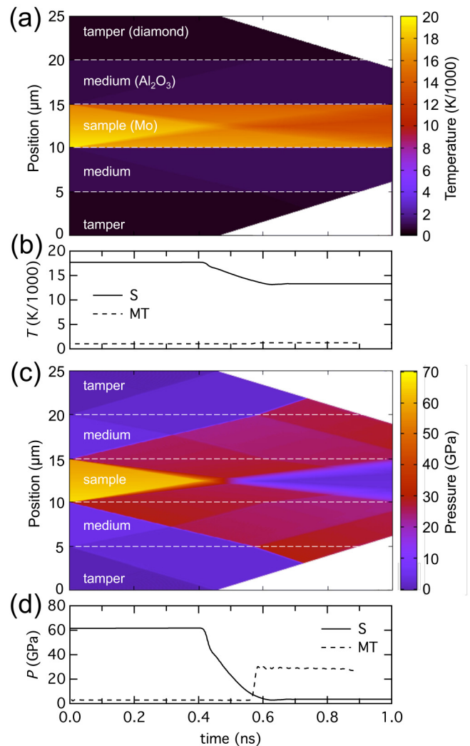
FIG. 10. One-dimensional radiation hydrocode (HYADES) model for the sample area of a target in first 10^{-9} s after irradiation. Here, a Mo sample ( 5 \mu\text{m} ), surrounded by \text{Al}_2\text{O}_3 medium layers ( 5 \mu\text{m} ) and diamond tampers (with thickness truncated to the displayed 5 \mu\text{m} ), is irradiated in a vacuum by 25 keV x rays (see Fig. 7, dark blue curves, for a finite element model of a comparable system, at a different initial temperature). X rays are incident from below. (a) Temperature throughout the simulated region (as a function of Lagrangian position and time). (b) Temperature histories at the sample center (S) and medium-tamper interface (MT). Temperature changes are adiabatic in nature on this timescale. (c) Pressures throughout the simulated region and time domain. (d) Pressure histories at the sample center and tamper surface. Regions where the simulation boundary interfered with the results were removed. The simulation makes a LTE approximation, which is suitable for treating these timescales. 52
