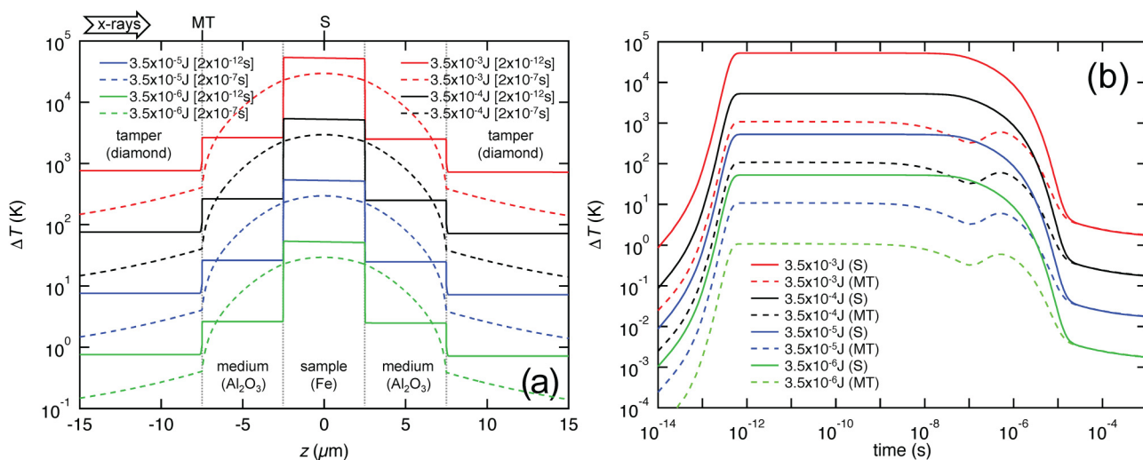
FIG. 4. Variance of thermal response with x-ray fluence (energy per pulse). (a) Temperature change vs position along the beam path center ( r = 0 ) in the sample region. (b) Temperature change vs time at sample center (S) and leading medium-tamper interface (MT). The black lines correspond to the standard simulation. Times are given in square brackets in seconds.
