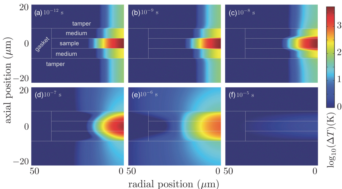
FIG. 3. Temperature change map in the r - z plane for the standard experiment at different times, showing the detailed behavior of the sample area. Lines show the boundaries between sample components (see Fig. 1).
