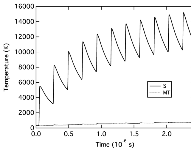
FIG. 12. Stepwise “isobaric” heating by x-ray pulses delivered in a pulse train. The standard FE model configuration is used with a 220 ns (4.5 MHz) pulse delay time assumed. Temperatures at the sample center (S) and medium-tamper interface (MT) are shown for the first 11 pulses. Pulse duration is increased to a few ns in this model to ensure numerical stability in the longer duration simulation.
