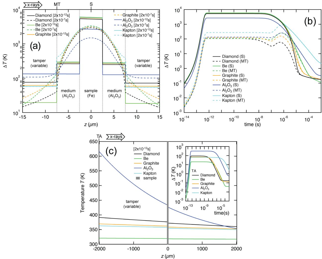
FIG. 8. Variance of thermal response with tamper material. (a) Temperature change vs position along the beam path center ( r = 0 ) in the sample region. (b) Temperature change vs time at sample center (S) and leading medium-tamper interface (MT). (c) Absolute temperature vs position along the beam path center ( r = 0 ) across whole target with inset showing temperature change vs time at the leading tamper free surface (TA). The black lines correspond to the standard simulation. Times are given in square brackets in seconds.
