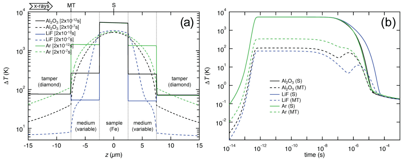
FIG. 9. Variance of thermal response with interfacial layer (medium) material. (a) Temperature change vs position along the beam path center ( r = 0 ) in the sample region. (b) Temperature change vs time at sample center (S) and leading medium-tamper interface (MT). The black lines correspond to the standard simulation. Times are given in square brackets in seconds.
