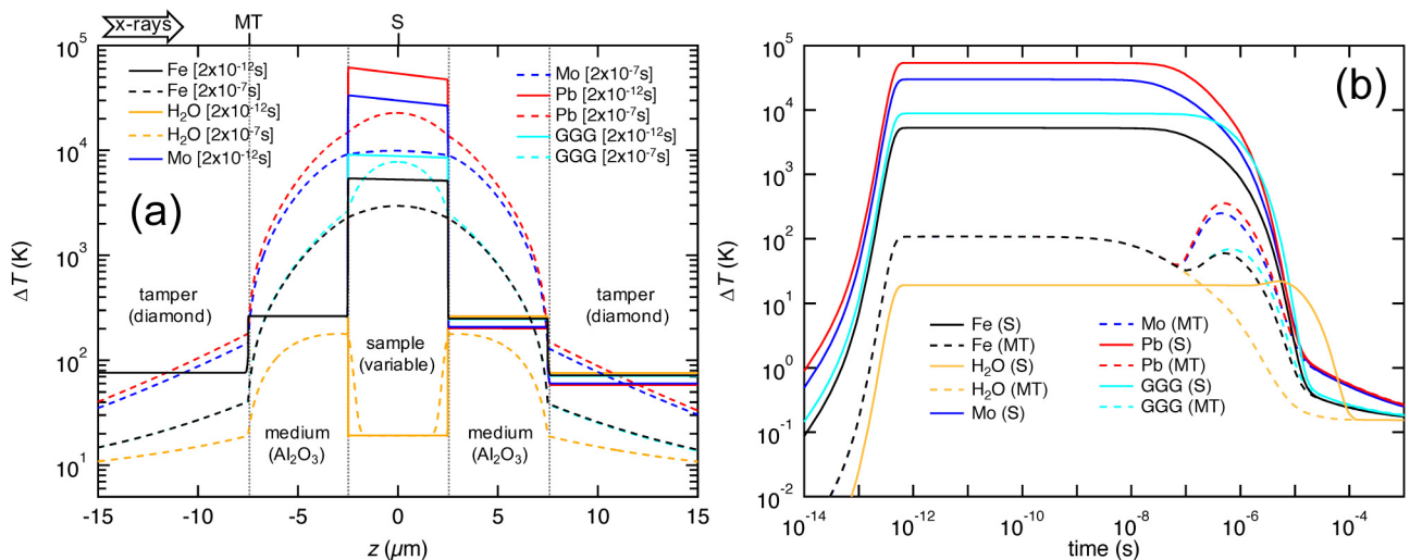
FIG. 7. Variance of thermal response with sample material. (a) Temperature change vs position along the beam path center ( r = 0 ) in the sample region. (b) Temperature change vs time at sample center (S) and leading medium-tamper interface (MT). The black lines correspond to the standard simulation. Times are given in square brackets in seconds.
