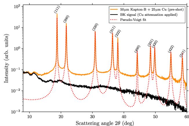
FIG. 3. Diffraction signal from an unshocked 25\text{-}\mu\text{m} thick Cu sample overcoated with 50\text{-}\mu\text{m} of Kapton, and, on the same scale, the diffraction signal from 50\text{-}\mu\text{m} Kapton with the x-ray attenuation due to the copper applied. Also shown is the sum of Voigt-profile fits to the Bragg peaks of the Cu sample.
